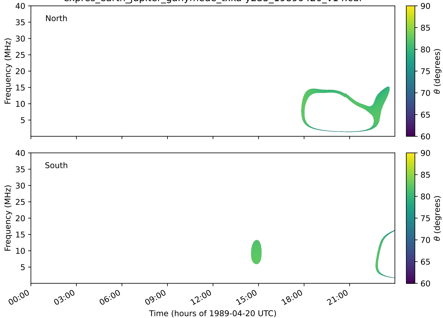
expres_earth_jupiter_ganymede_txka-y235_19890420_v14.cdf
