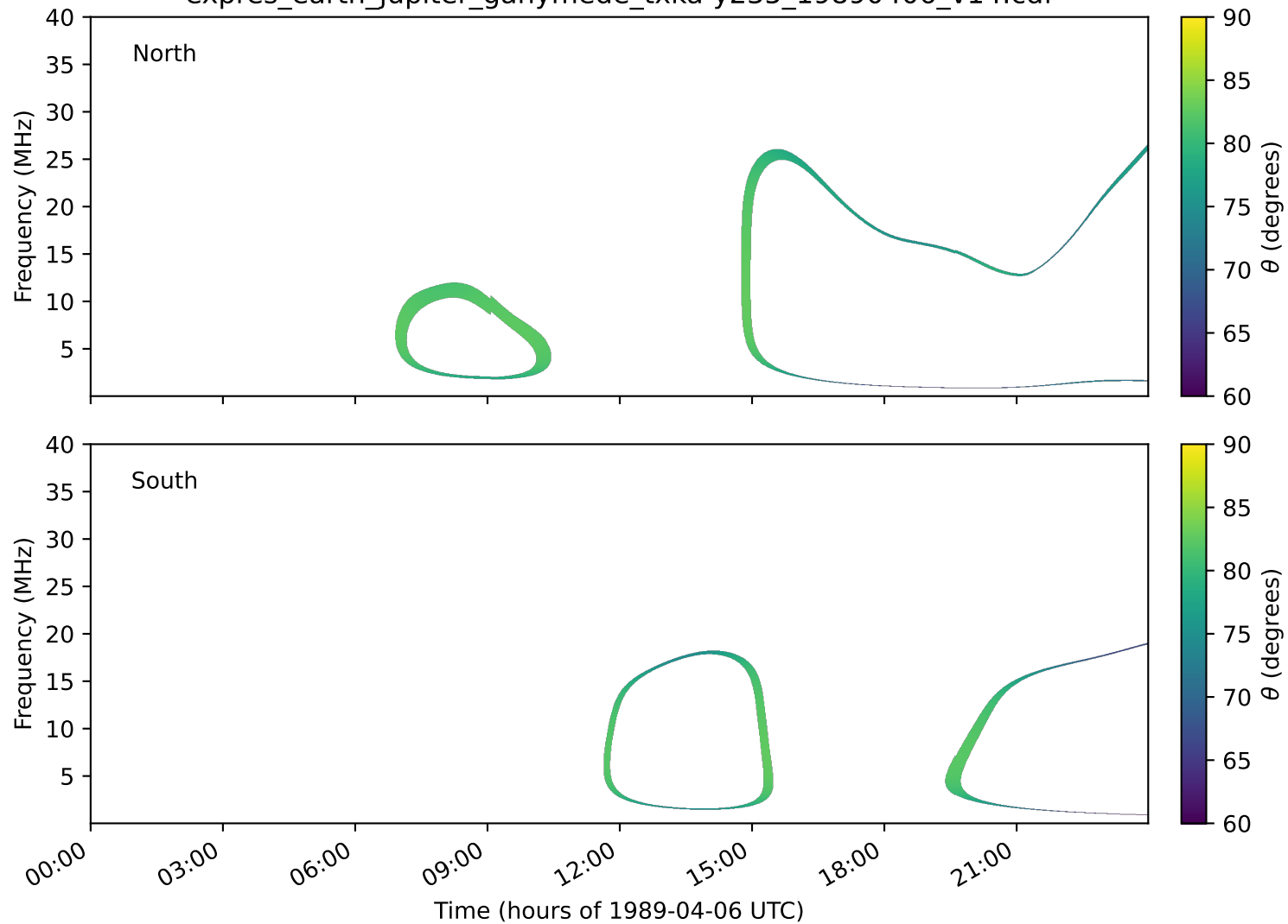
expres_earth_jupiter_ganymede_txka-y235_19890406_v14.cdf
