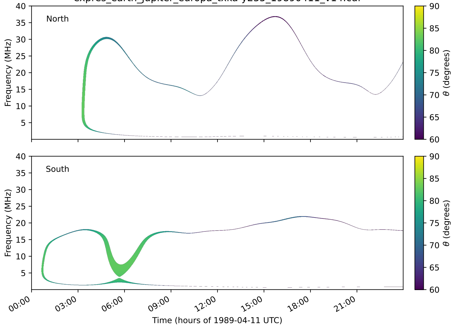
expres_earth_jupiter_europa_txka-y235_19890411_v14.cdf
