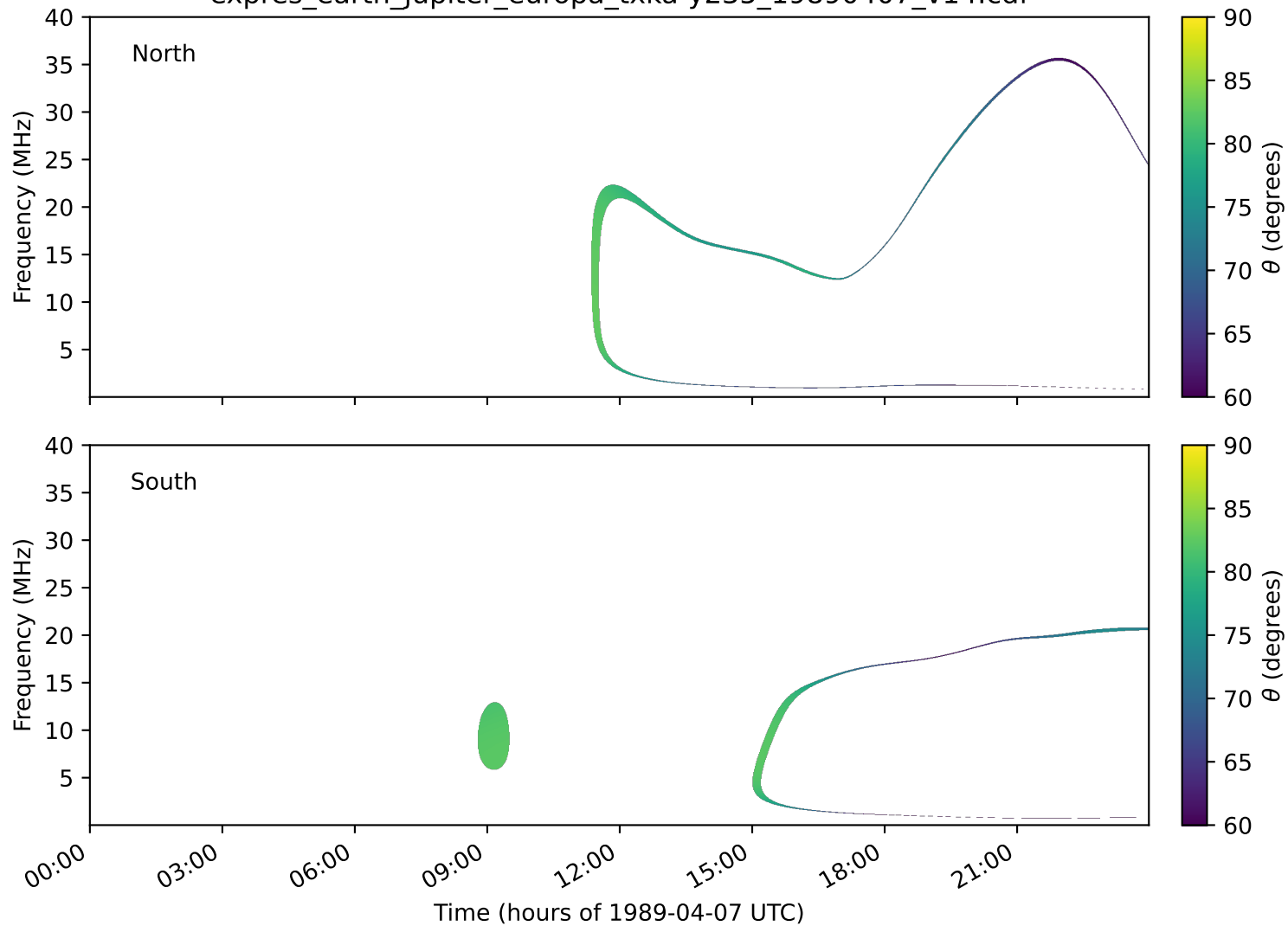
expres_earth_jupiter_europa_txka-y235_19890407_v14.cdf
