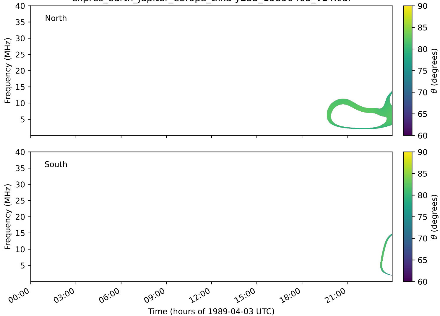
expres_earth_jupiter_europa_txka-y235_19890403_v14.cdf
