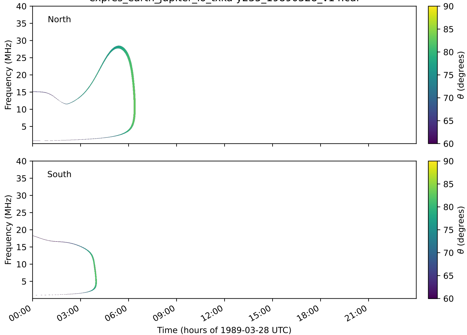
expres_earth_jupiter_io_txka-y235_19890328_v14.cdf
