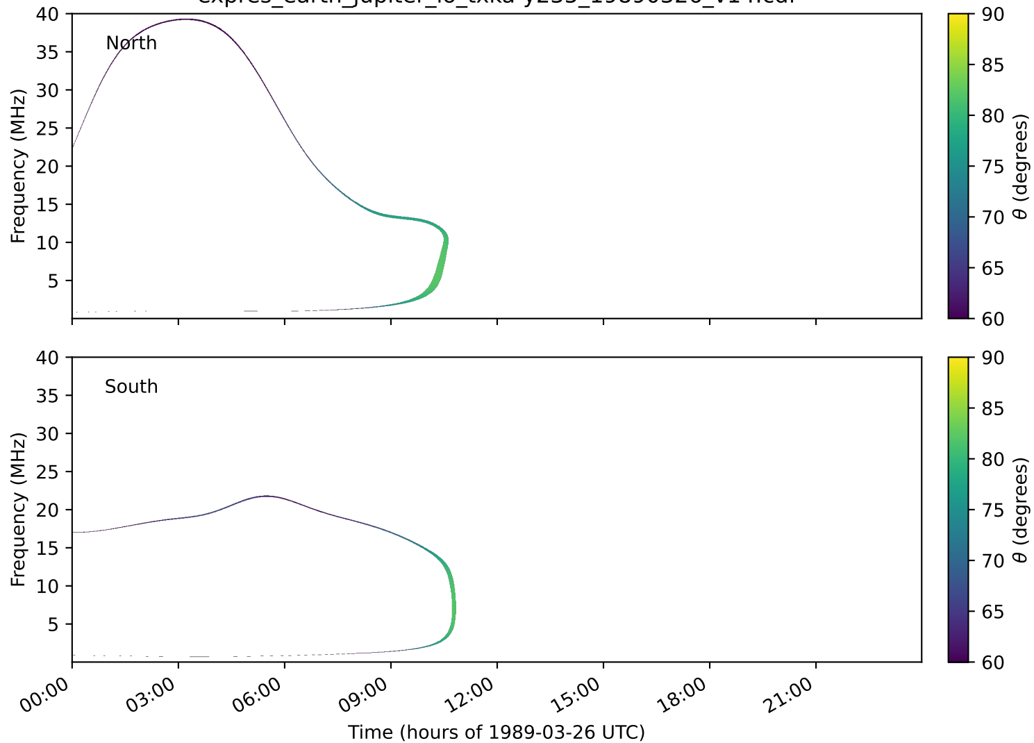
expres_earth_jupiter_io_txka-y235_19890326_v14.cdf
