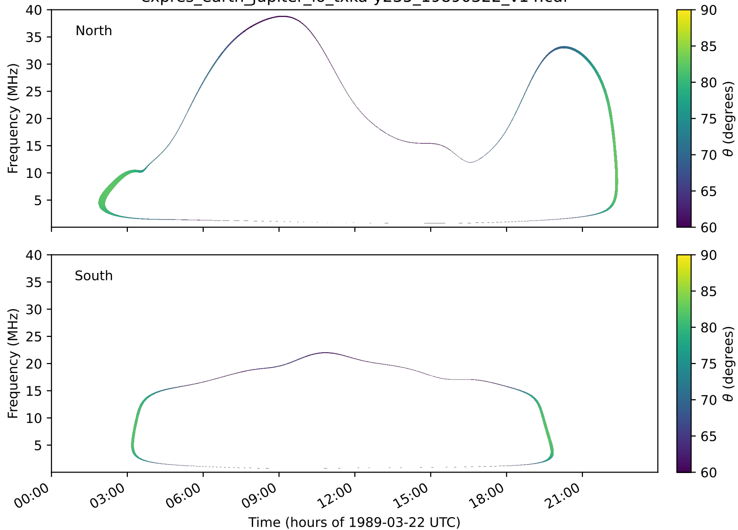
expres_earth_jupiter_io_txka-y235_19890322_v14.cdf
