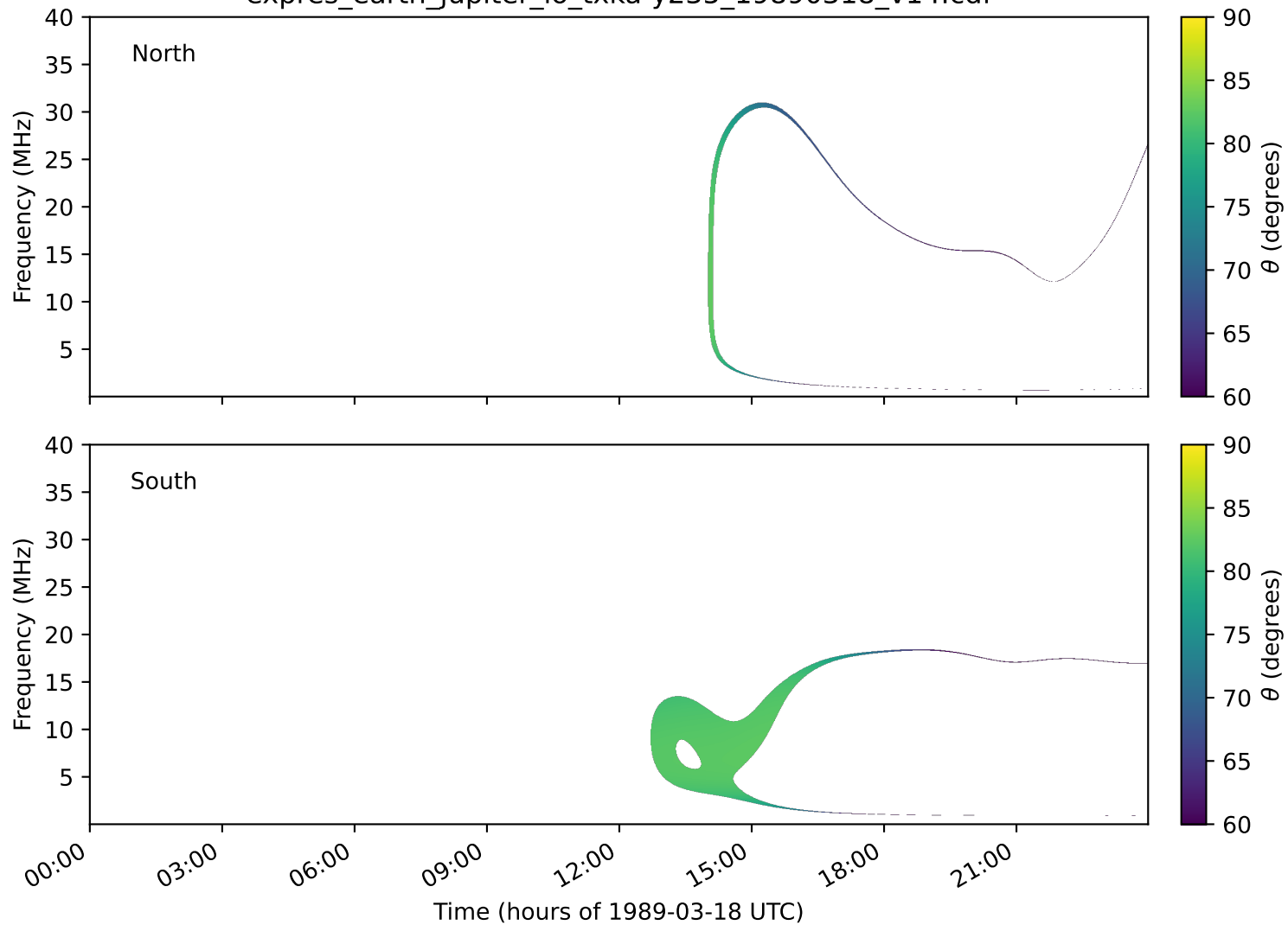
expres_earth_jupiter_io_txka-y235_19890318_v14.cdf
