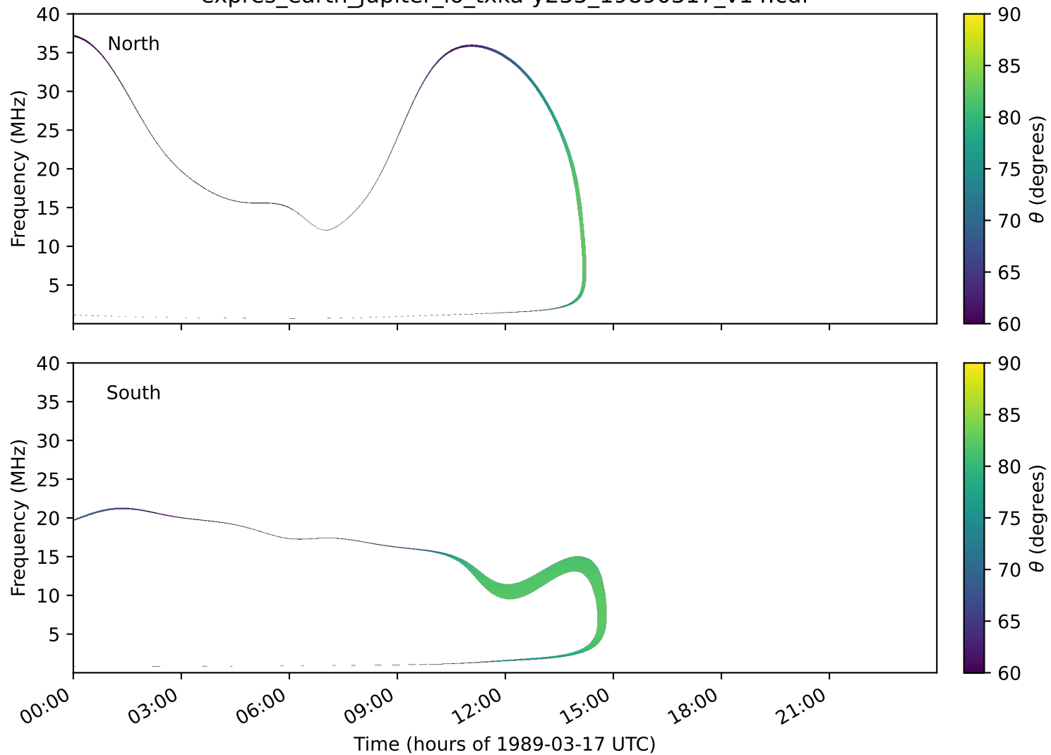
expres_earth_jupiter_io_txka-y235_19890317_v14.cdf
