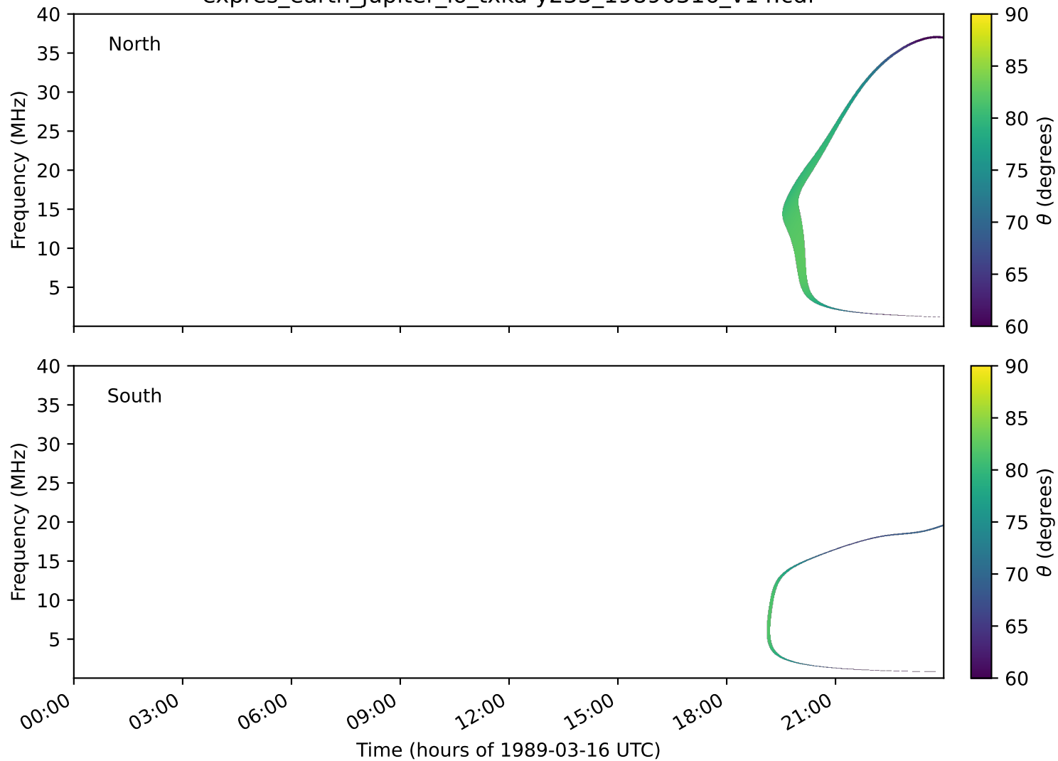
expres_earth_jupiter_io_txka-y235_19890316_v14.cdf
