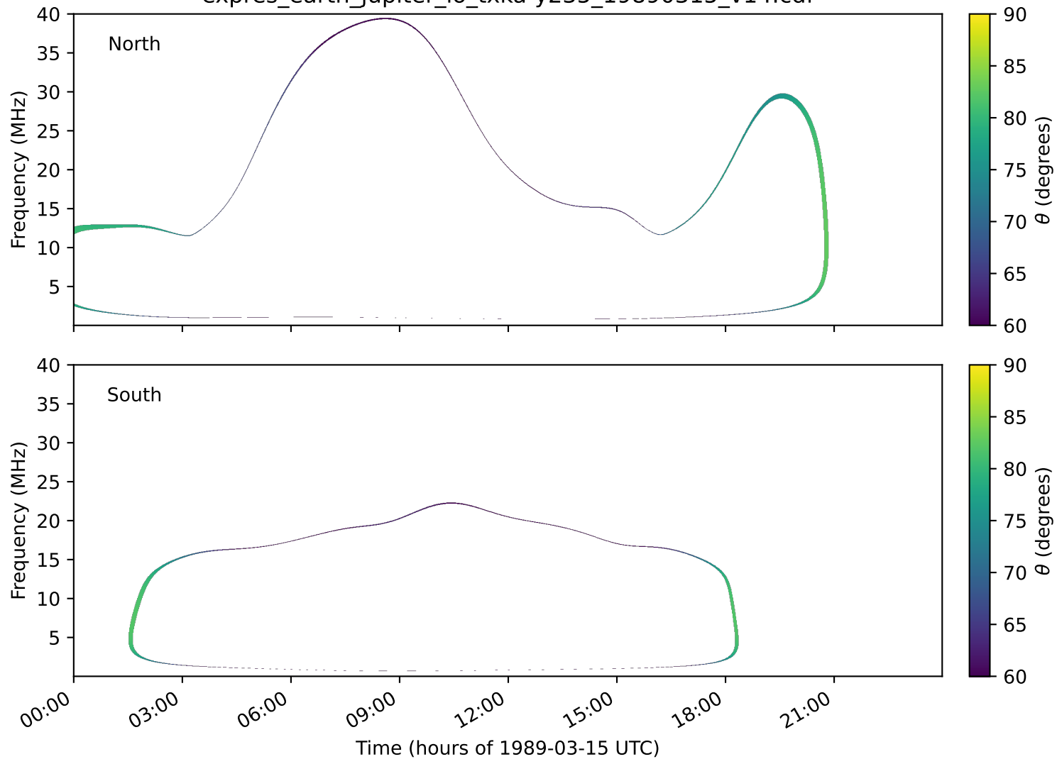
expres_earth_jupiter_io_txka-y235_19890315_v14.cdf
