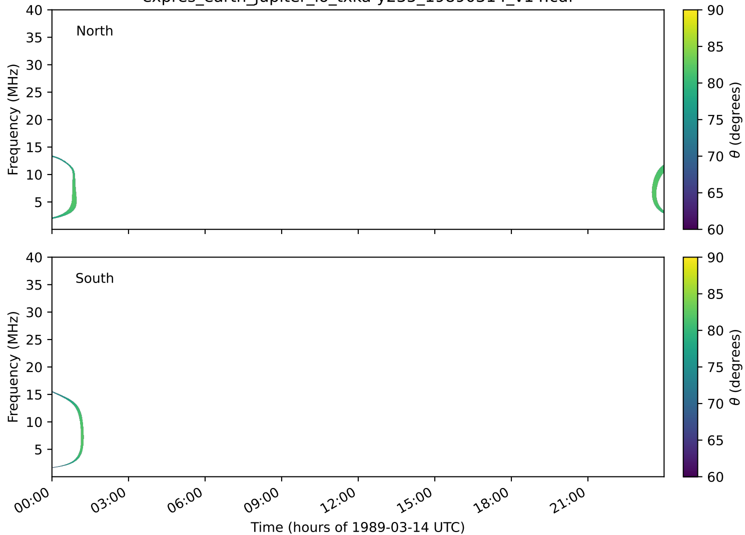
expres_earth_jupiter_io_txka-y235_19890314_v14.cdf
