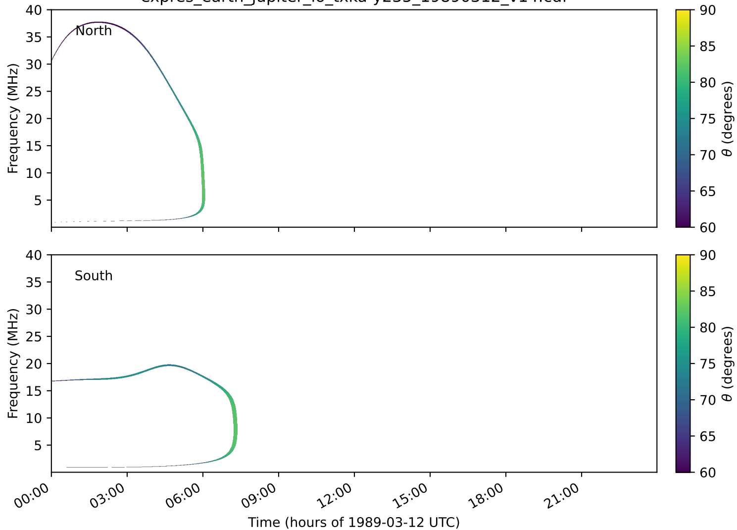
expres_earth_jupiter_io_txka-y235_19890312_v14.cdf
