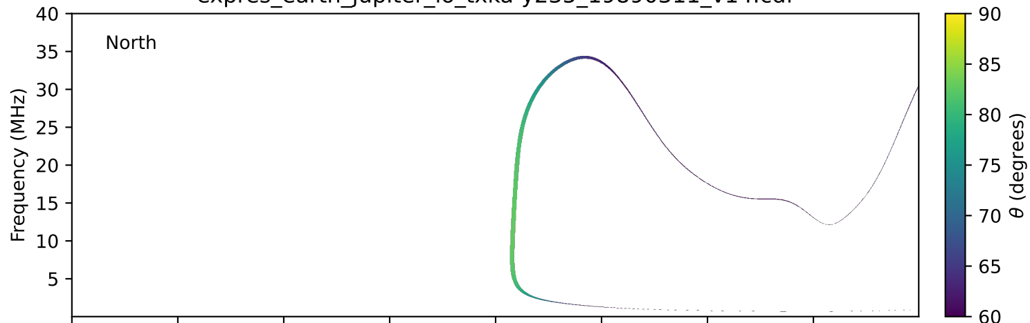
expres_earth_jupiter_io_txka-y235_19890311_v14.cdf
