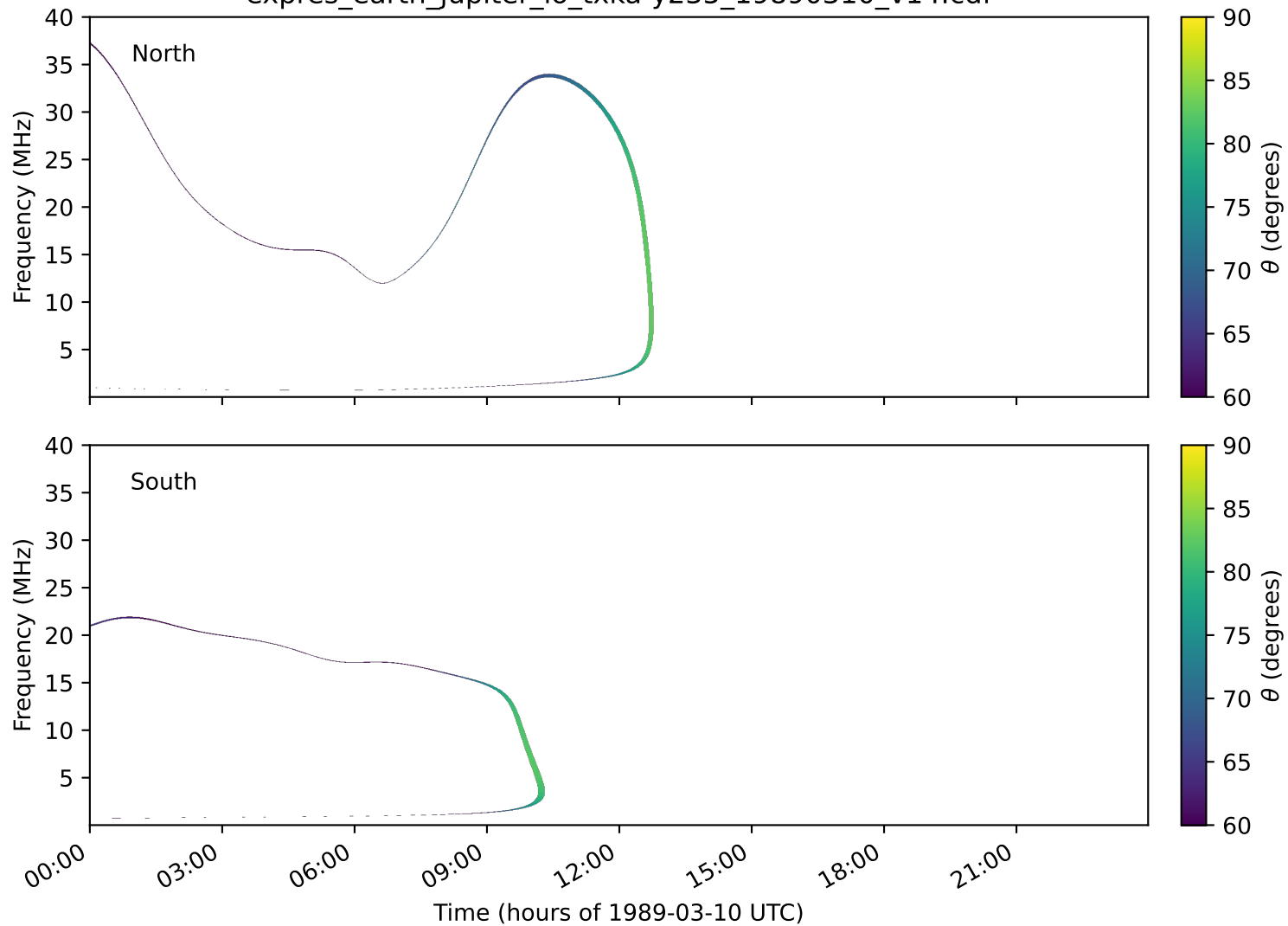
expres_earth_jupiter_io_txka-y235_19890310_v14.cdf
