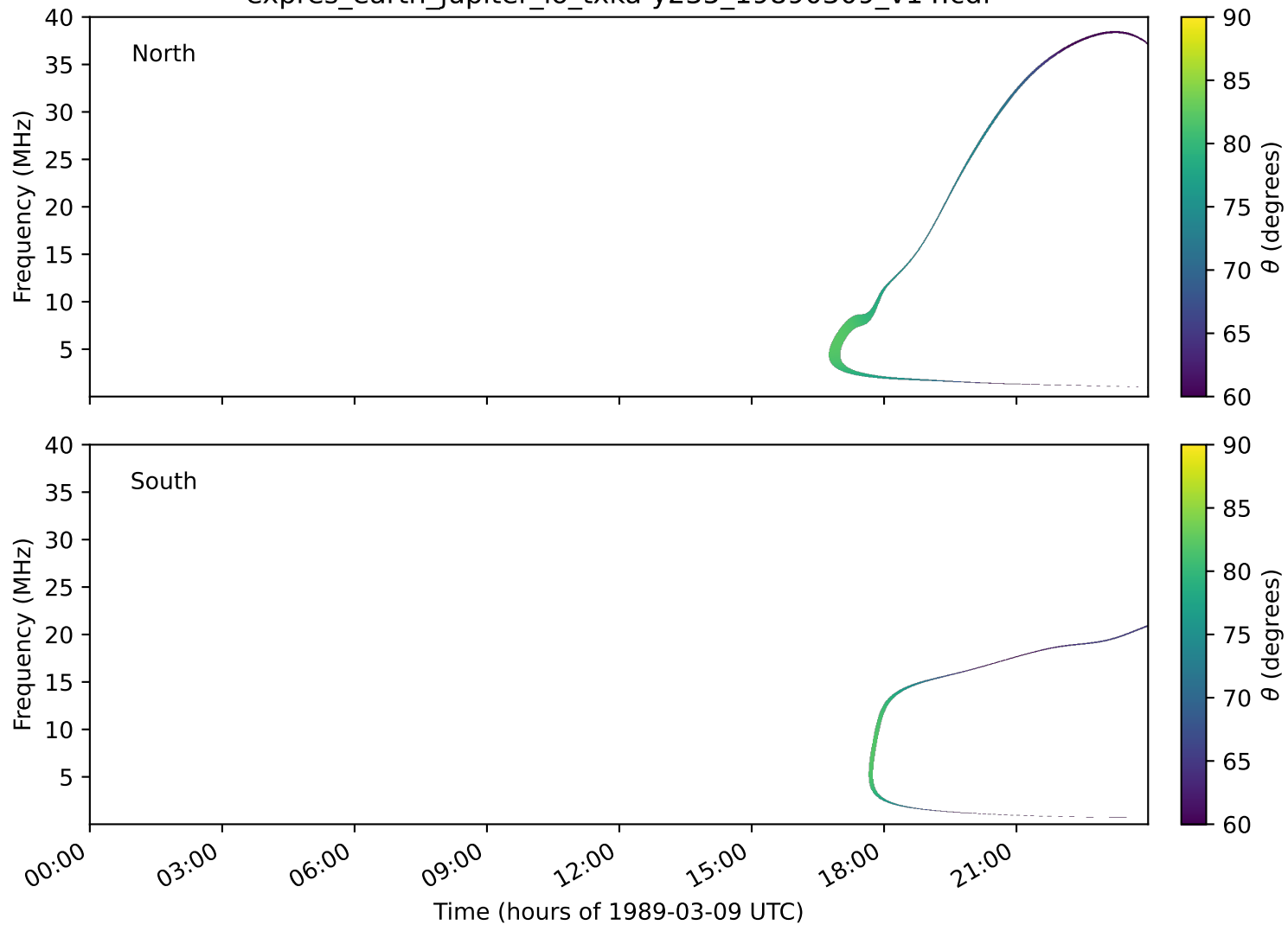
expres_earth_jupiter_io_txka-y235_19890309_v14.cdf
