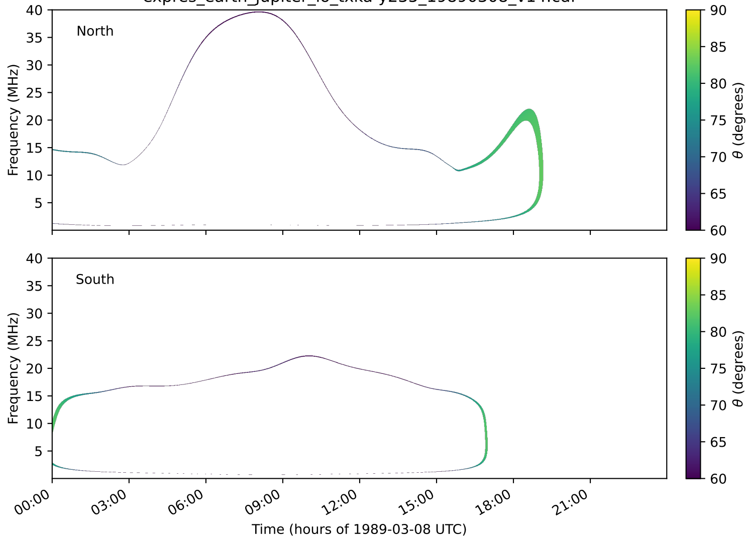
expres_earth_jupiter_io_txka-y235_19890308_v14.cdf
