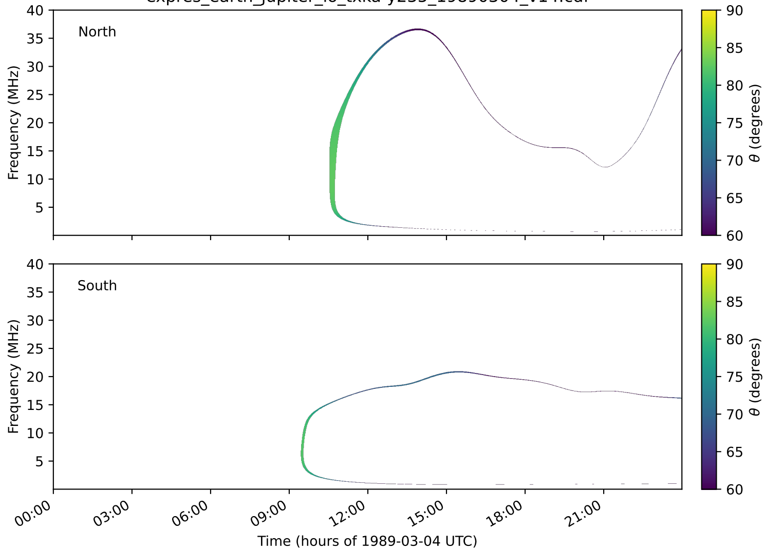
expres_earth_jupiter_io_txka-y235_19890304_v14.cdf
