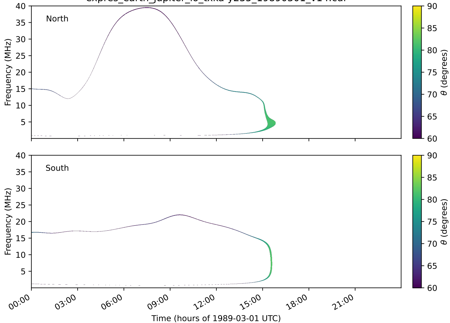
expres_earth_jupiter_io_txka-y235_19890301_v14.cdf
