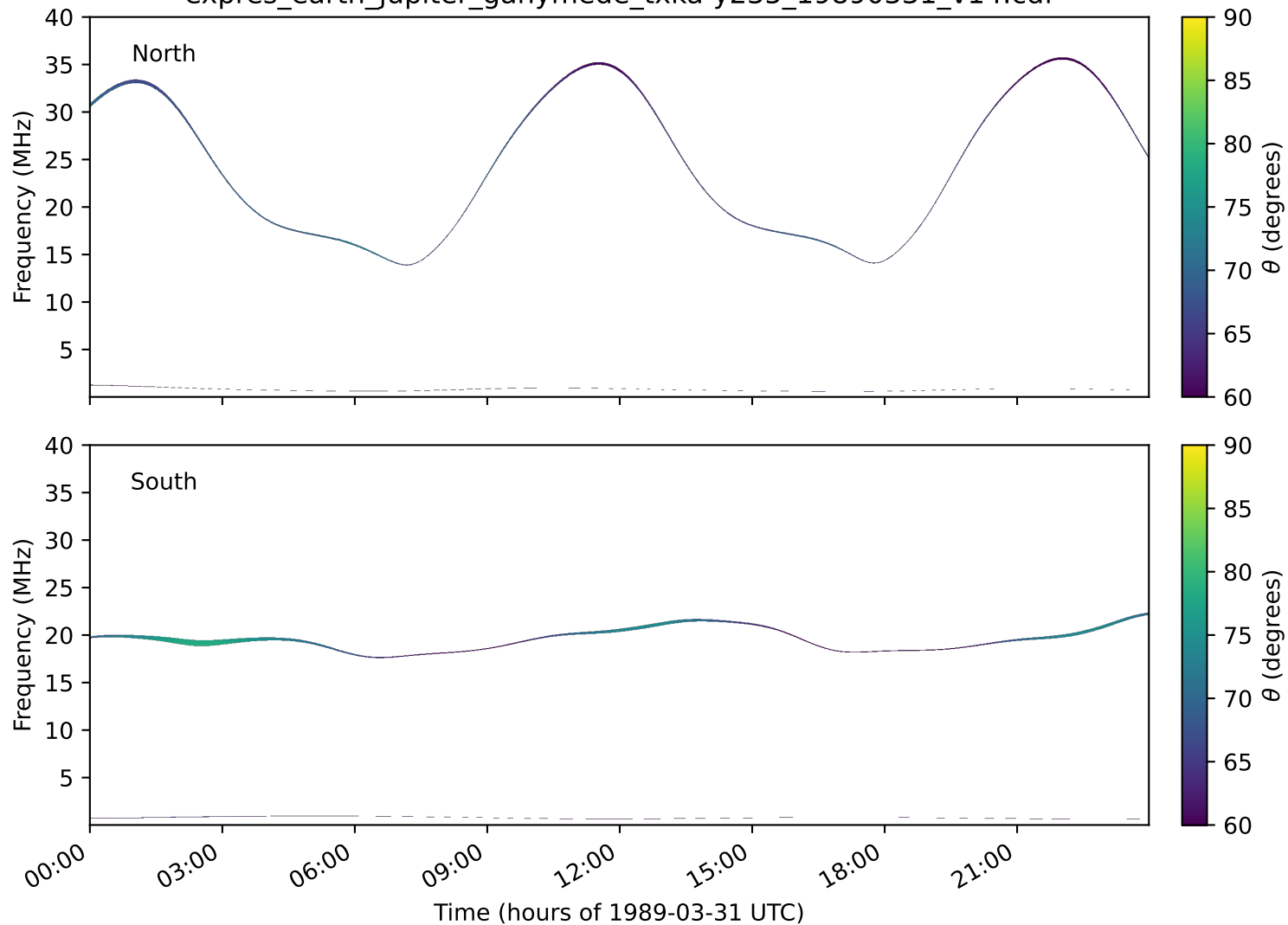
expres_earth_jupiter_ganymede_txka-y235_19890331_v14.cdf
