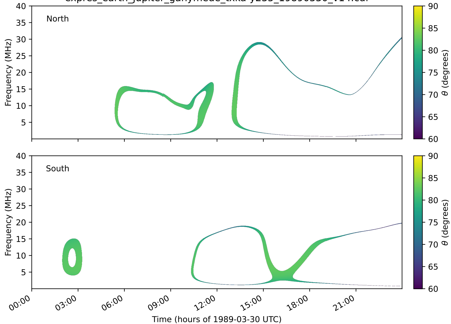
expres_earth_jupiter_ganymede_txka-y235_19890330_v14.cdf
