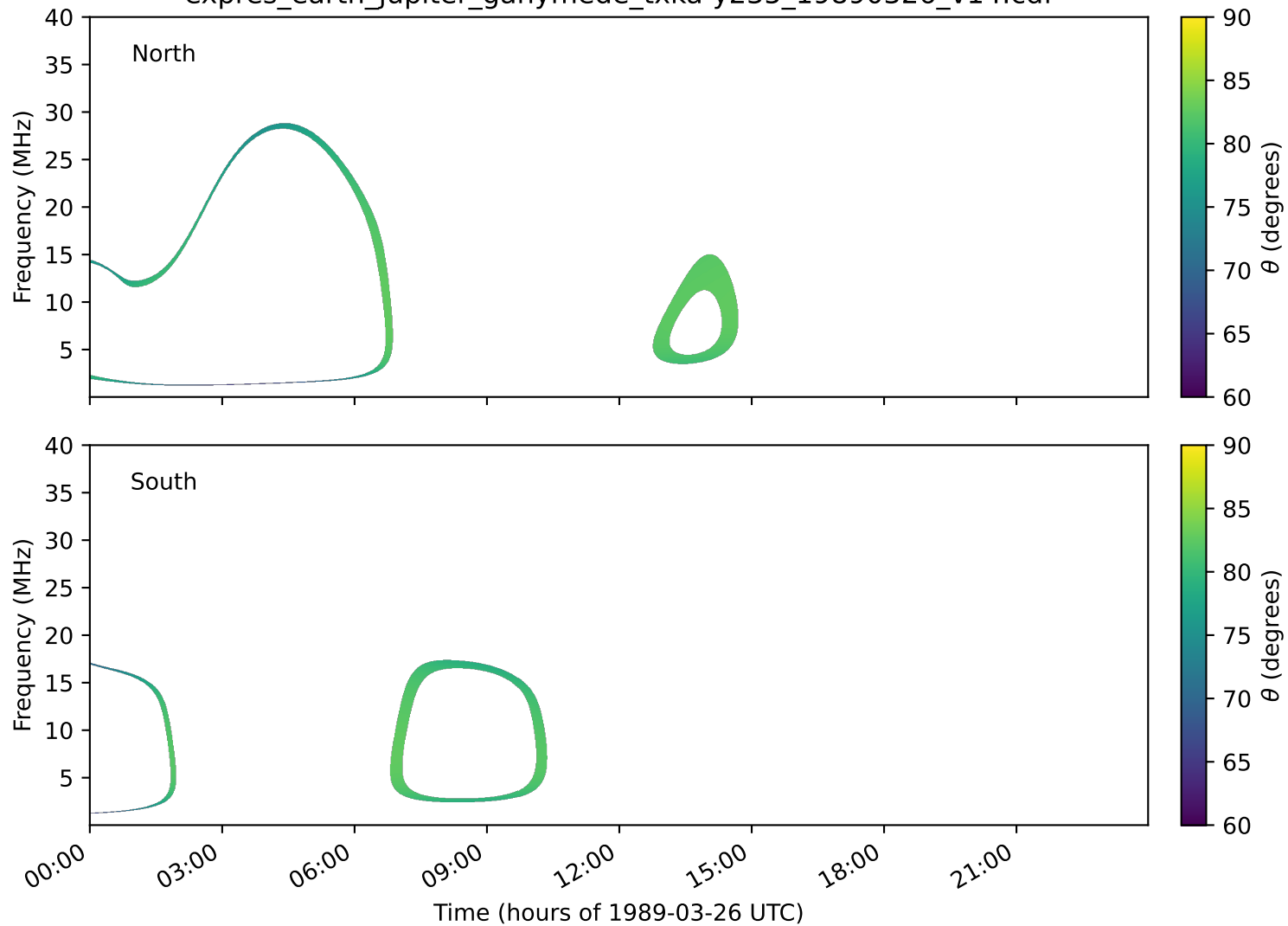
expres_earth_jupiter_ganymede_txka-y235_19890326_v14.cdf
