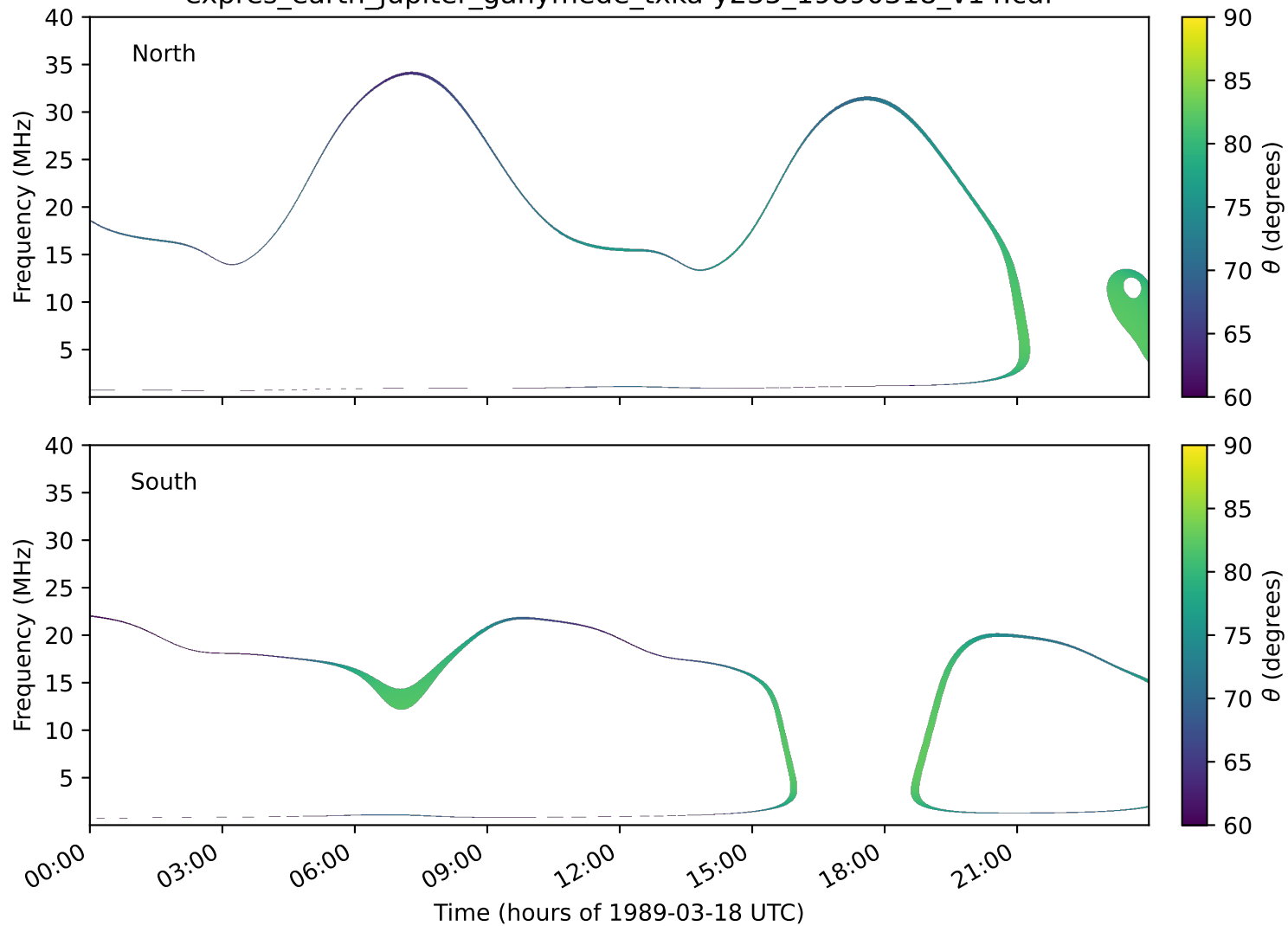
expres_earth_jupiter_ganymede_txka-y235_19890318_v14.cdf
