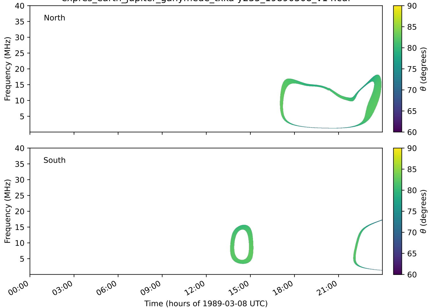
expres_earth_jupiter_ganymede_txka-y235_19890308_v14.cdf
