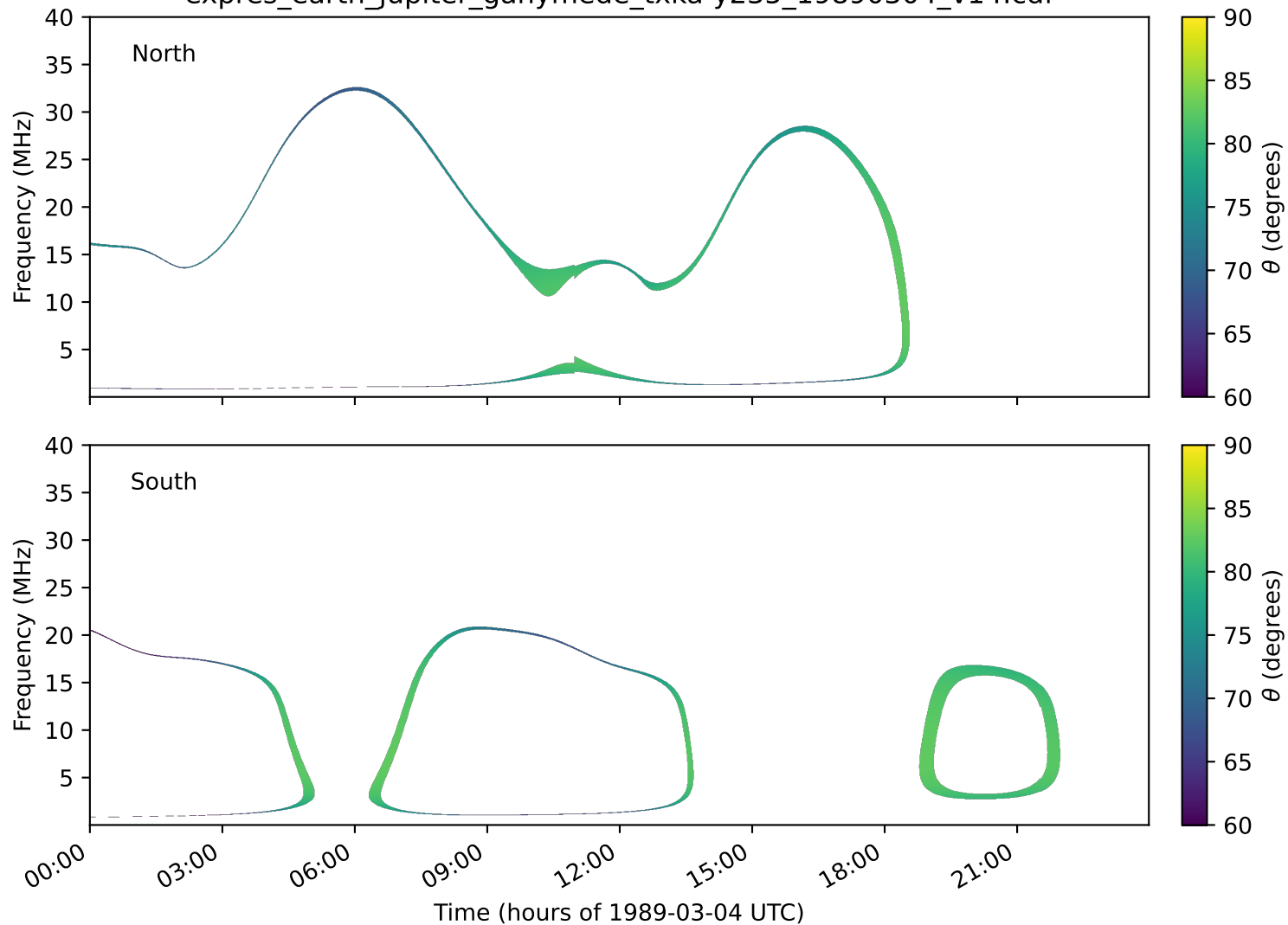
expres_earth_jupiter_ganymede_txka-y235_19890304_v14.cdf
