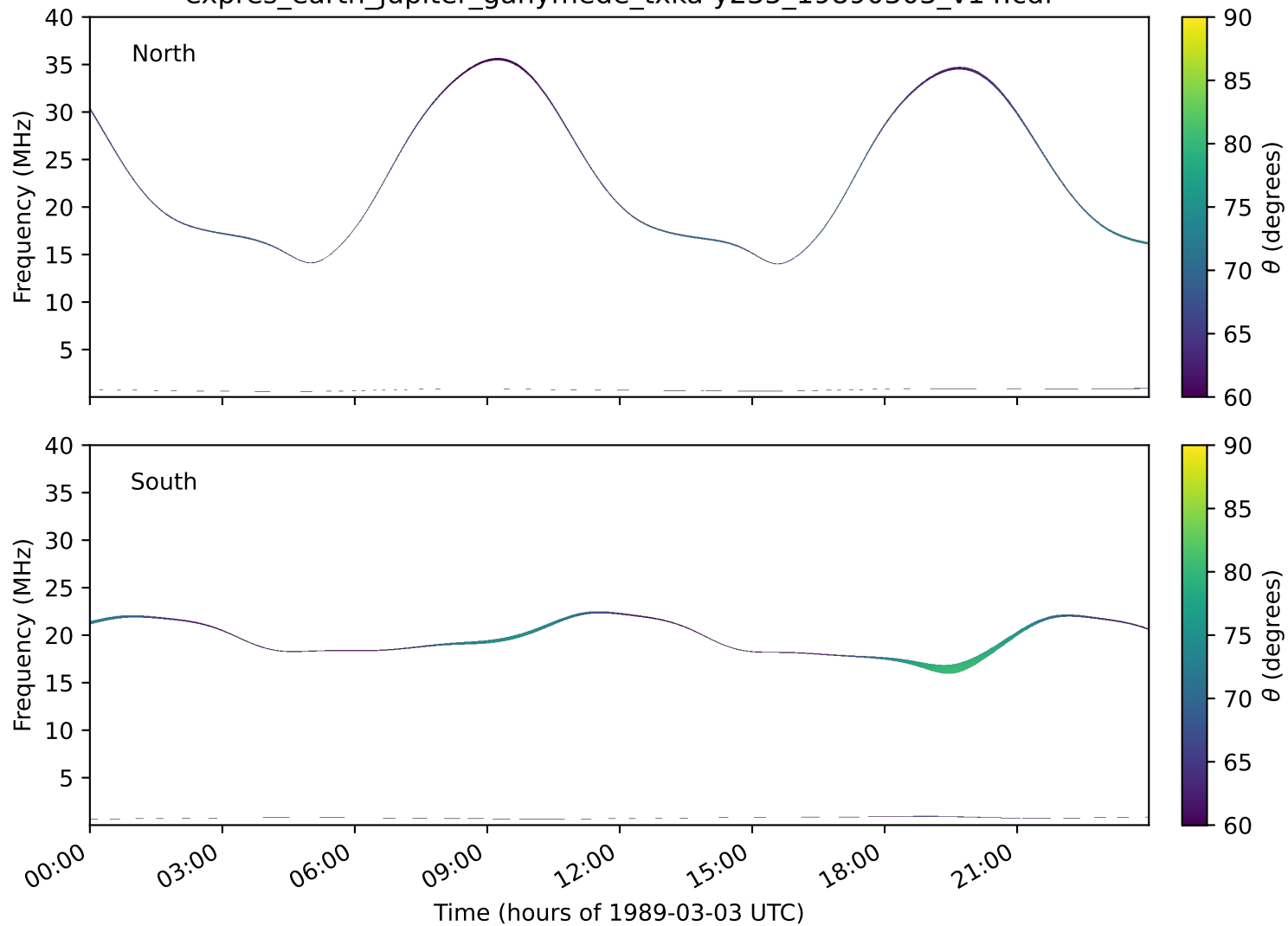
expres_earth_jupiter_ganymede_txka-y235_19890303_v14.cdf
