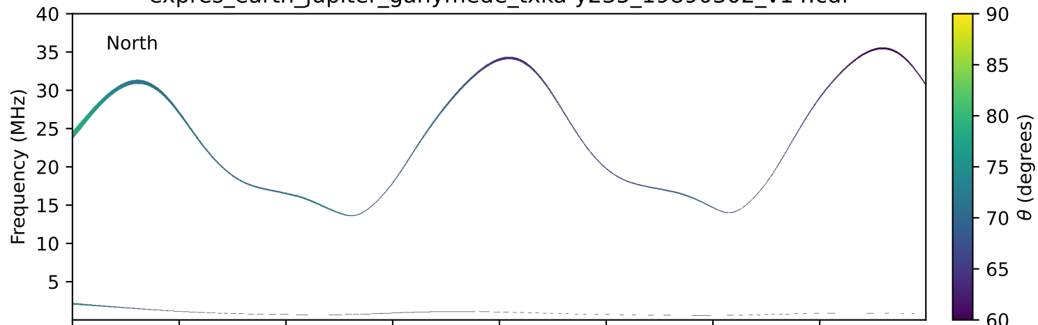
expres_earth_jupiter_ganymede_txka-y235_19890302_v14.cdf
