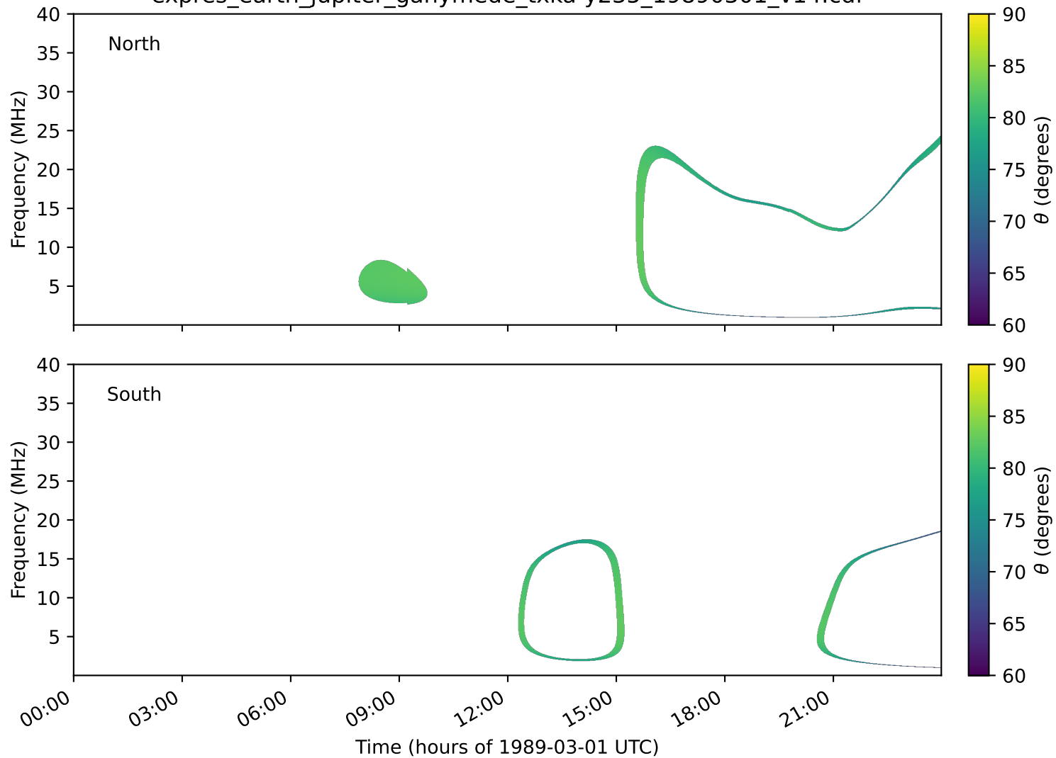
expres_earth_jupiter_ganymede_txka-y235_19890301_v14.cdf
