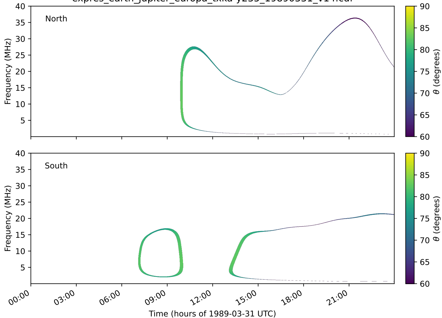
expres_earth_jupiter_europa_txka-y235_19890331_v14.cdf
