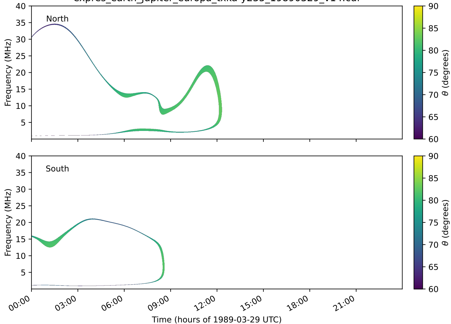
expres_earth_jupiter_europa_txka-y235_19890329_v14.cdf
