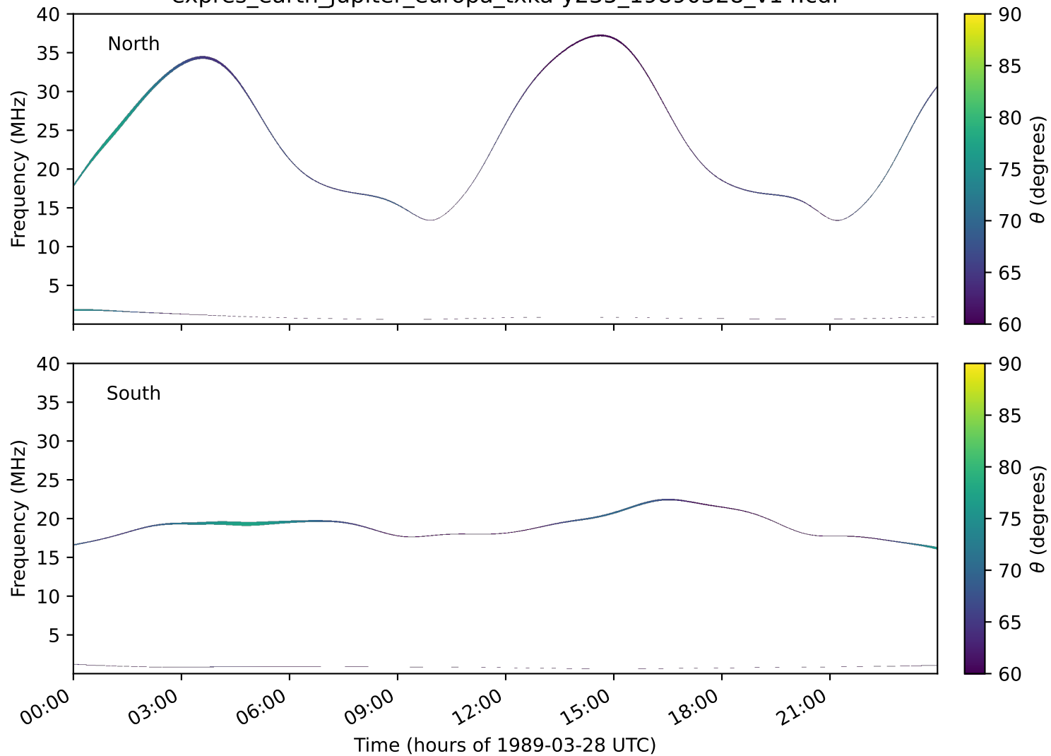
expres_earth_jupiter_europa_txka-y235_19890328_v14.cdf
