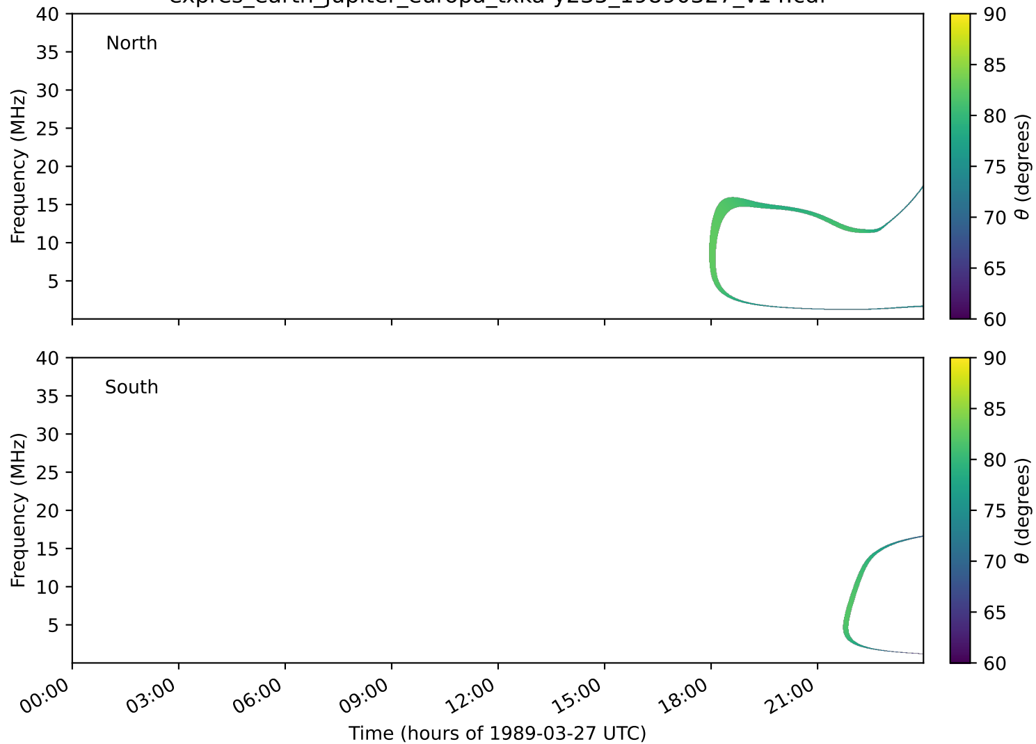
expres_earth_jupiter_europa_txka-y235_19890327_v14.cdf
