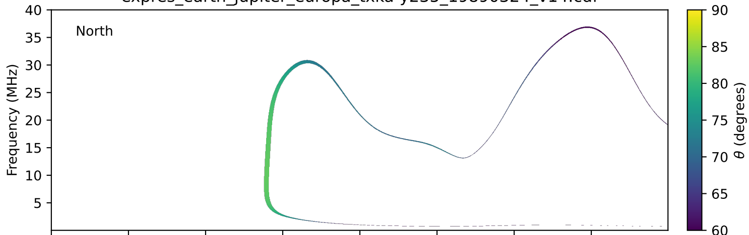
expres_earth_jupiter_europa_txka-y235_19890324_v14.cdf
