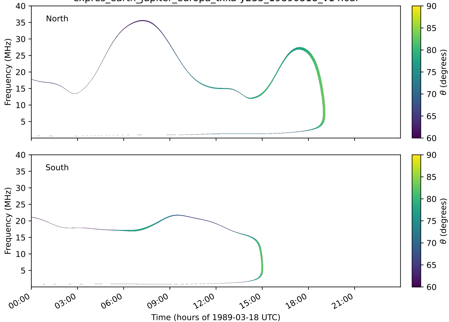
expres_earth_jupiter_europa_txka-y235_19890318_v14.cdf
