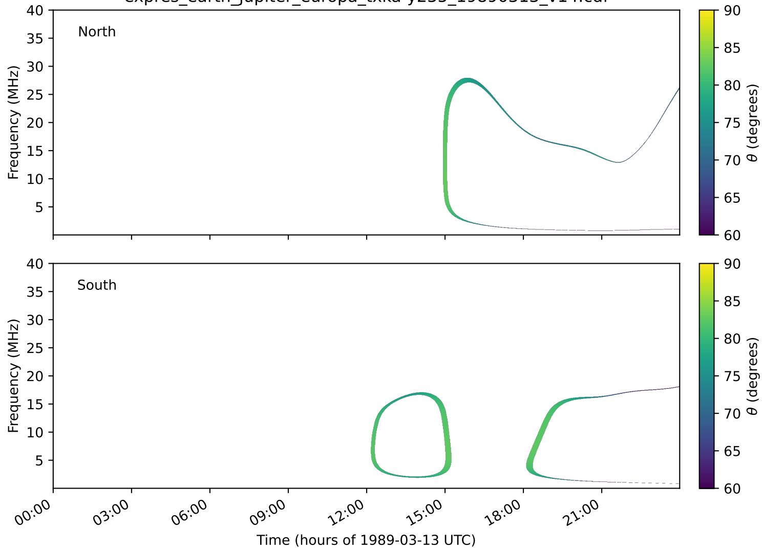
expres_earth_jupiter_europa_txka-y235_19890313_v14.cdf
