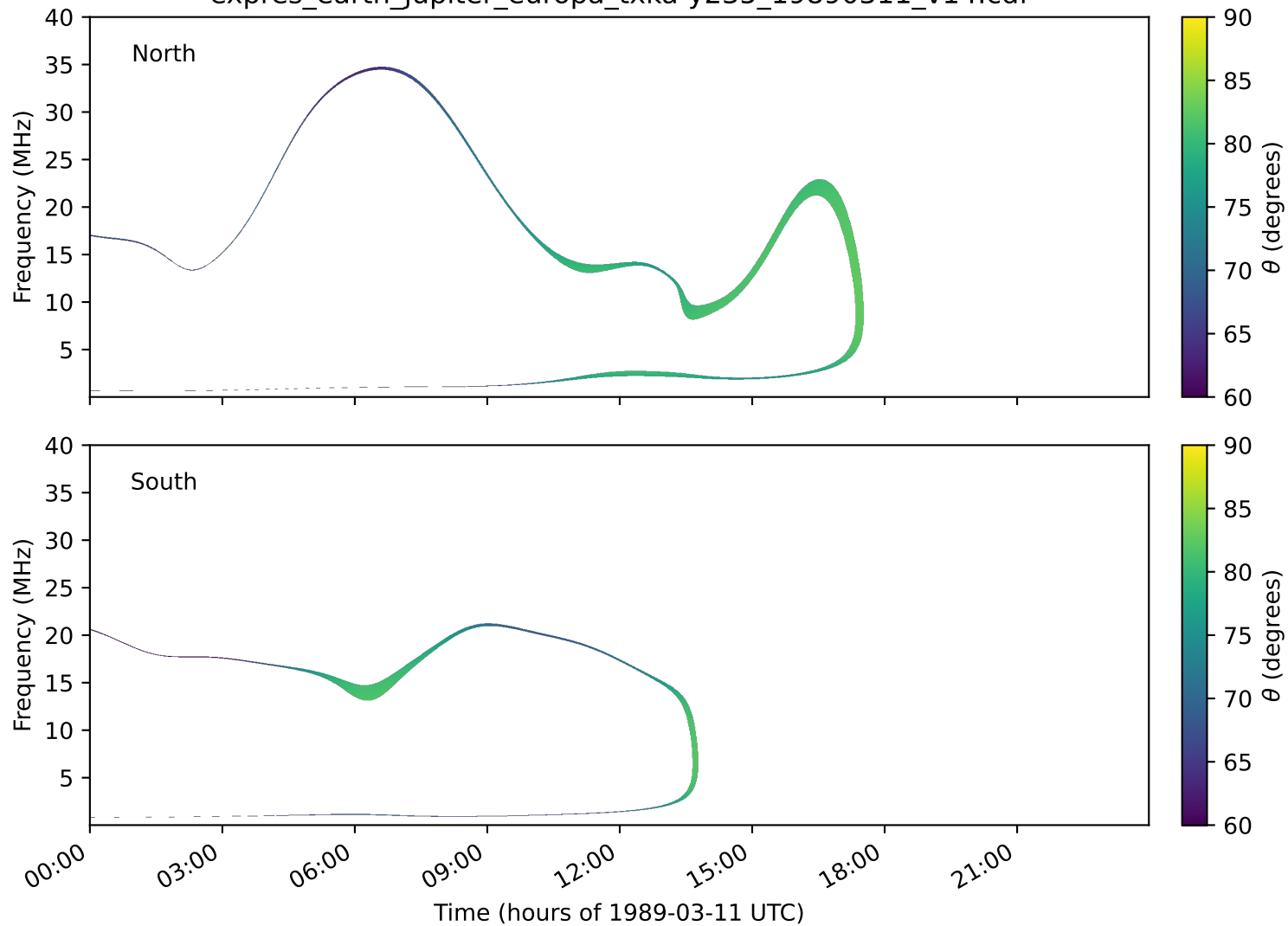
expres_earth_jupiter_europa_txka-y235_19890311_v14.cdf
