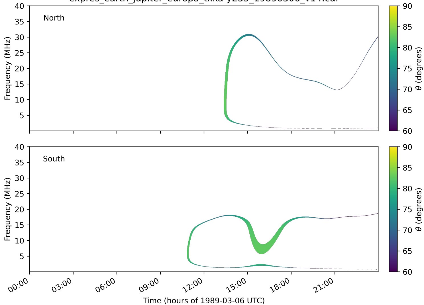
expres_earth_jupiter_europa_txka-y235_19890306_v14.cdf
