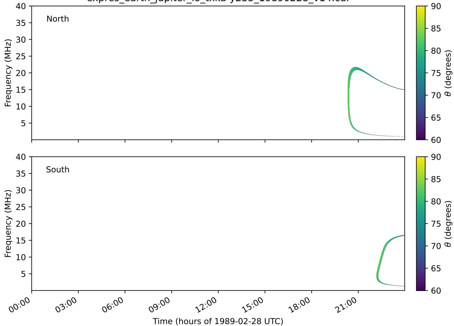
expres_earth_jupiter_io_txka-y235_19890228_v14.cdf
