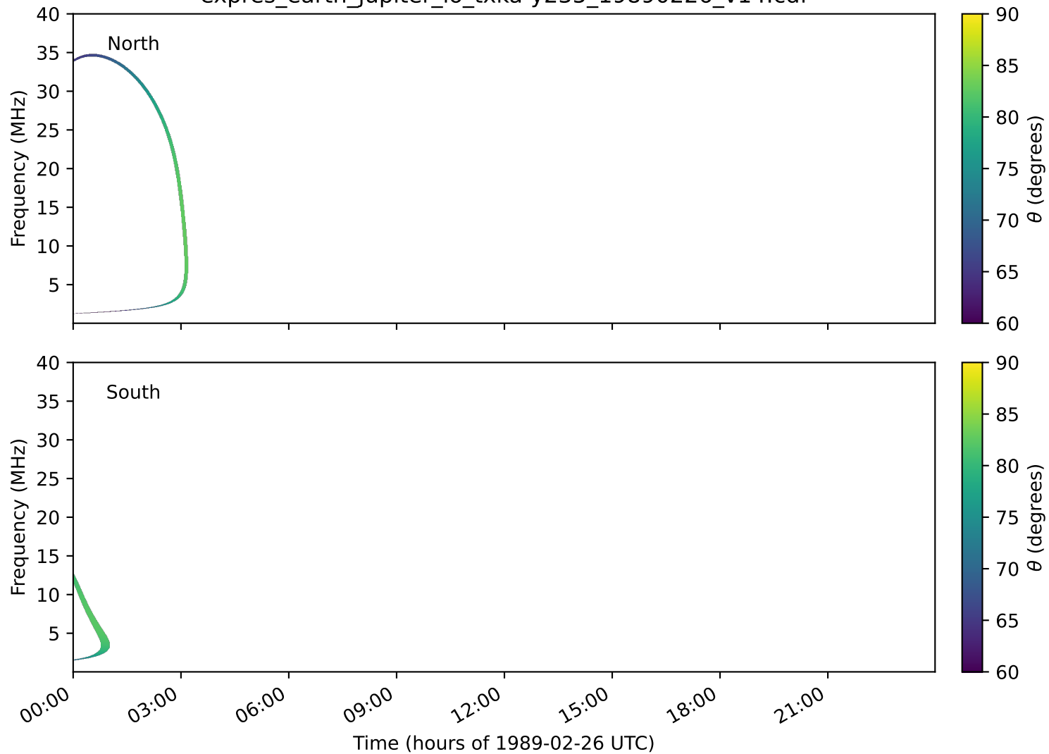
expres_earth_jupiter_io_txka-y235_19890226_v14.cdf
