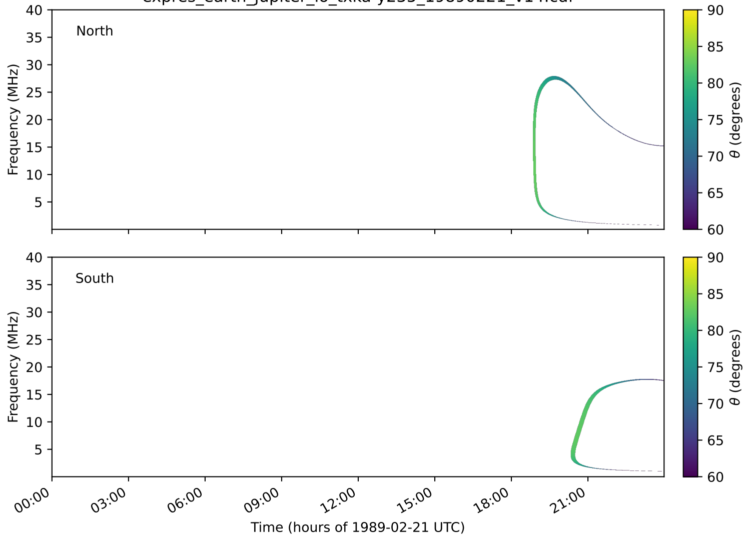
expres_earth_jupiter_io_txka-y235_19890221_v14.cdf
