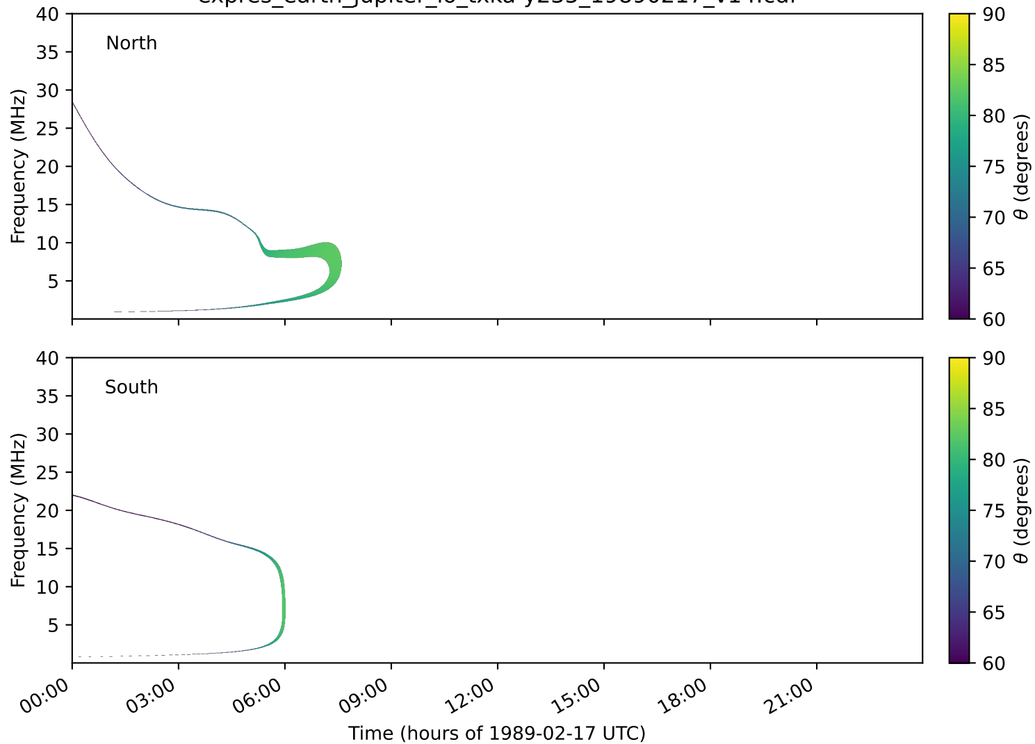
expres_earth_jupiter_io_txka-y235_19890217_v14.cdf
