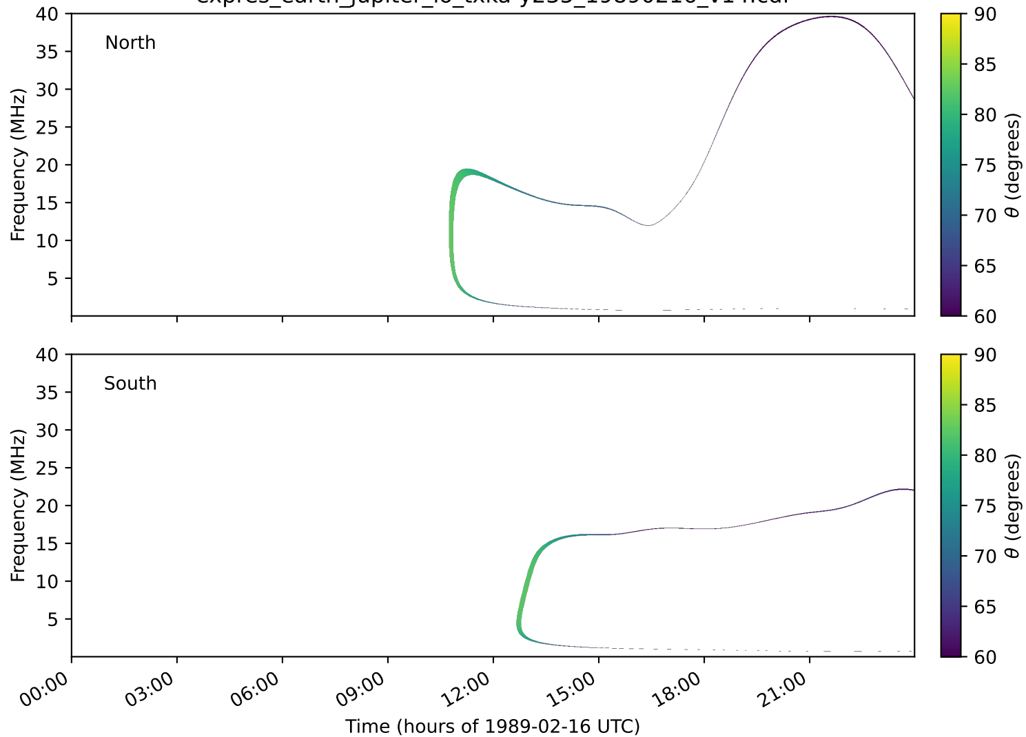
expres_earth_jupiter_io_txka-y235_19890216_v14.cdf
