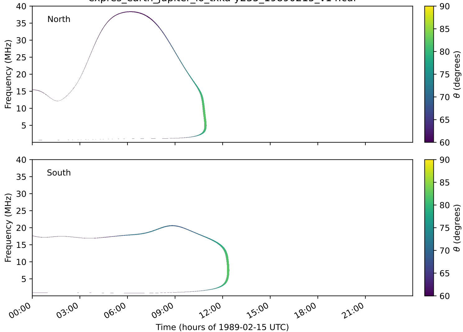
expres_earth_jupiter_io_txka-y235_19890215_v14.cdf
