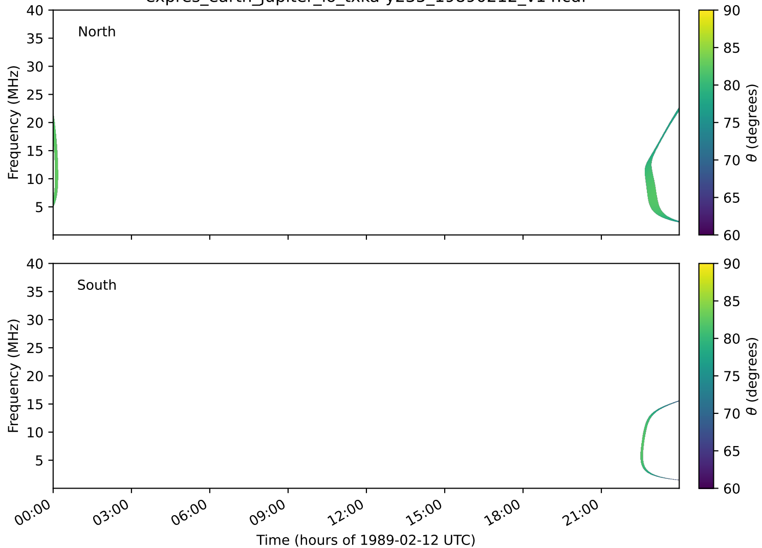
expres_earth_jupiter_io_txka-y235_19890212_v14.cdf
