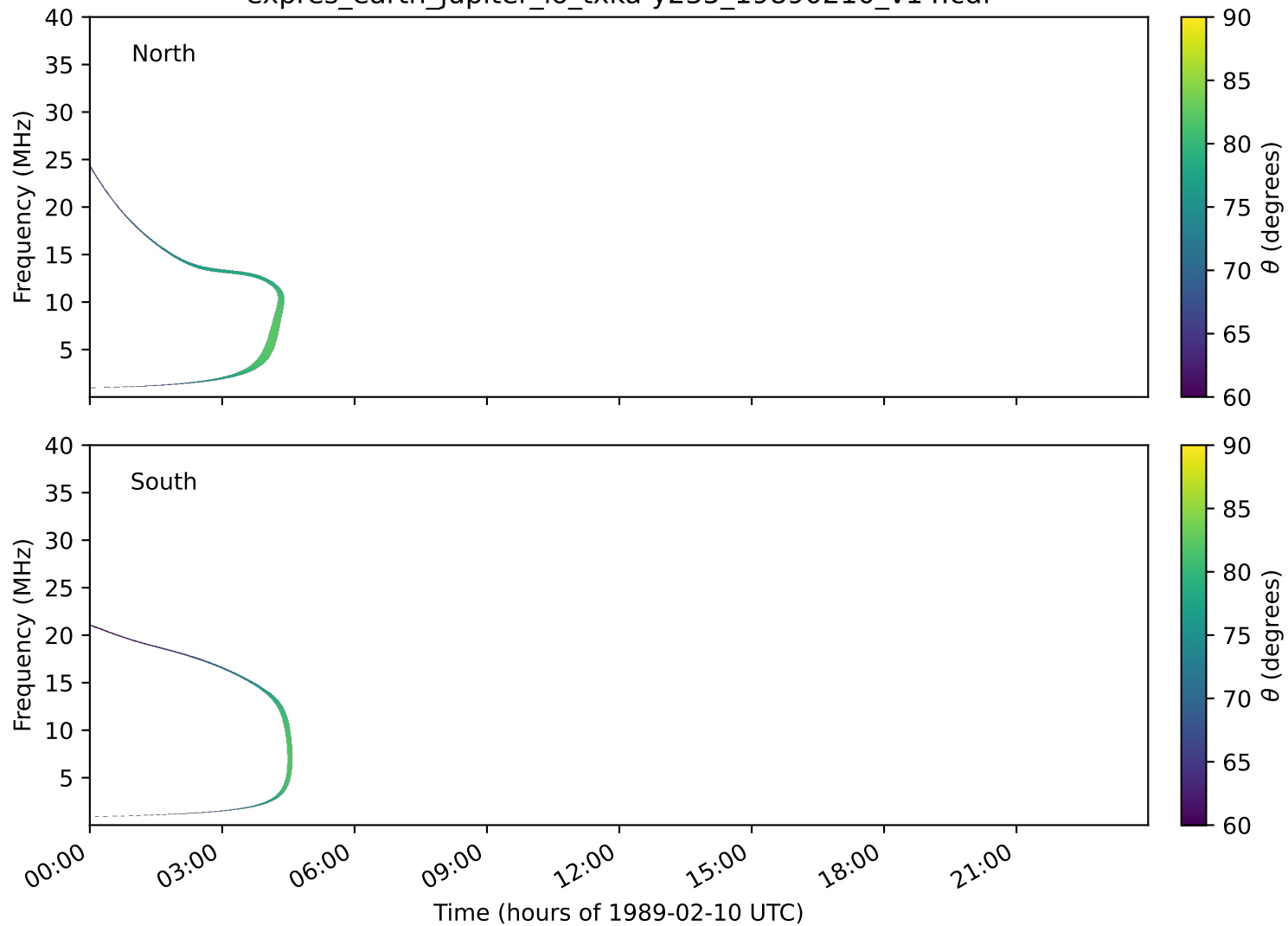
expres_earth_jupiter_io_txka-y235_19890210_v14.cdf
