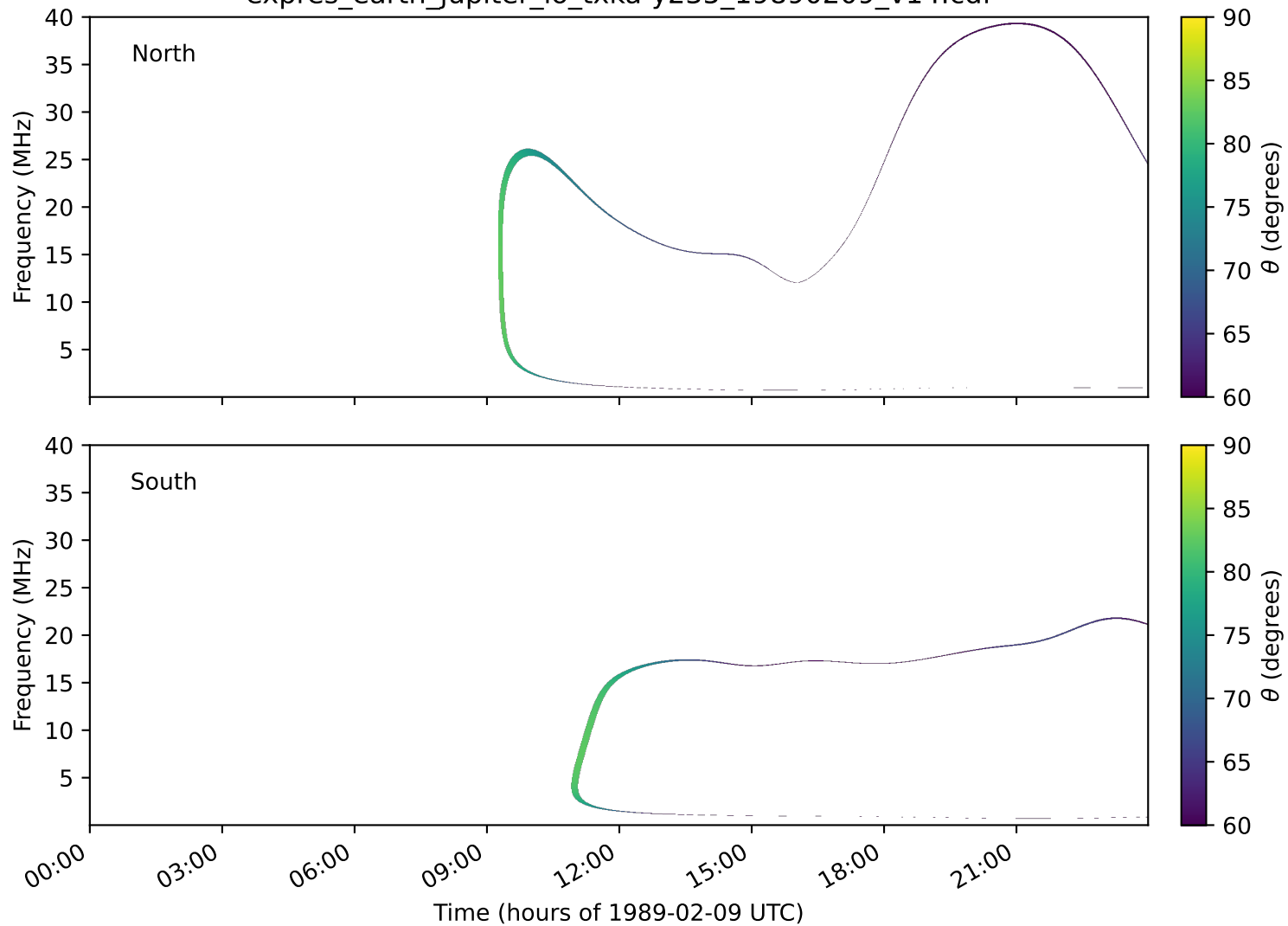
expres_earth_jupiter_io_txka-y235_19890209_v14.cdf
