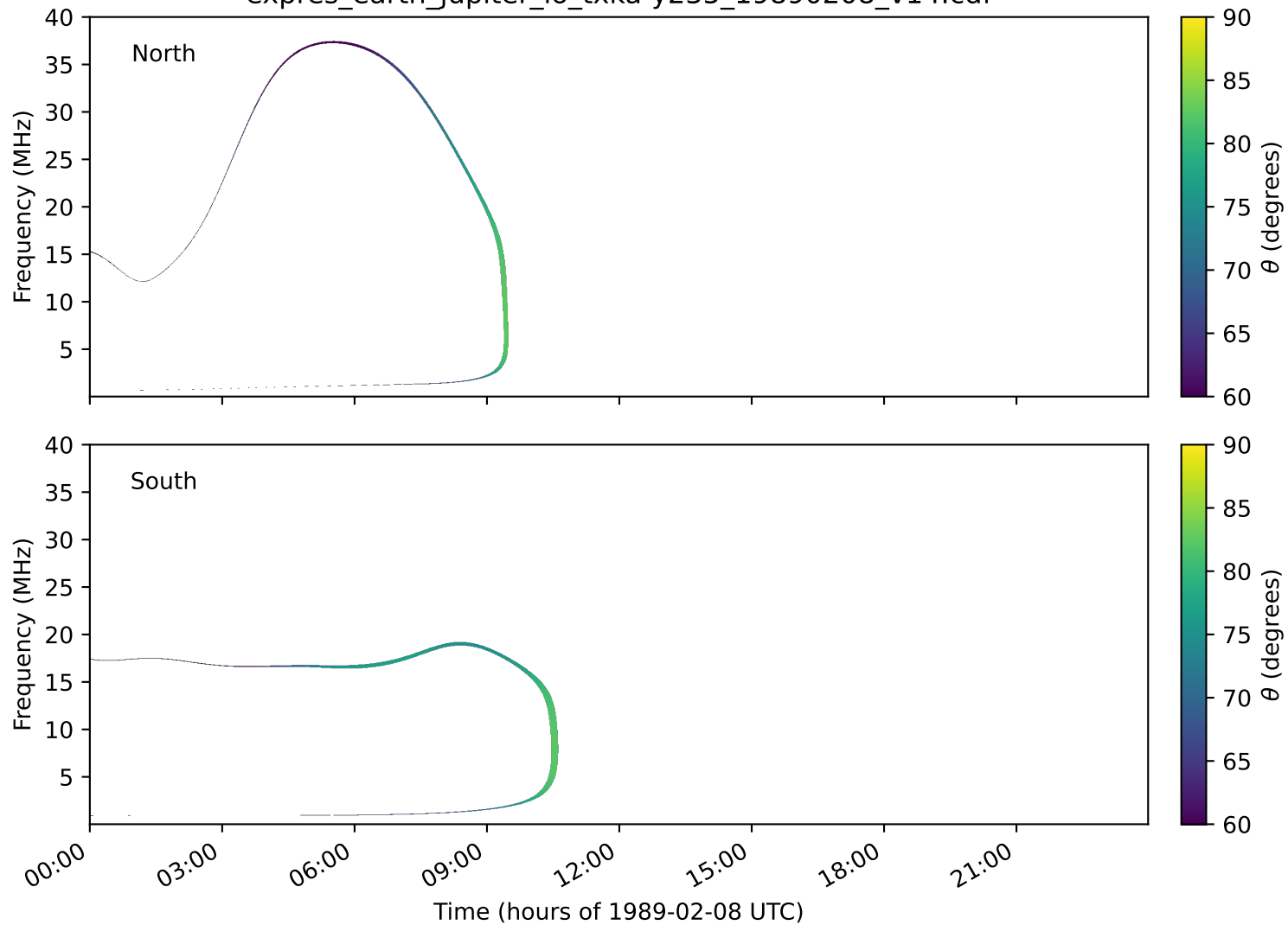
expres_earth_jupiter_io_txka-y235_19890208_v14.cdf
