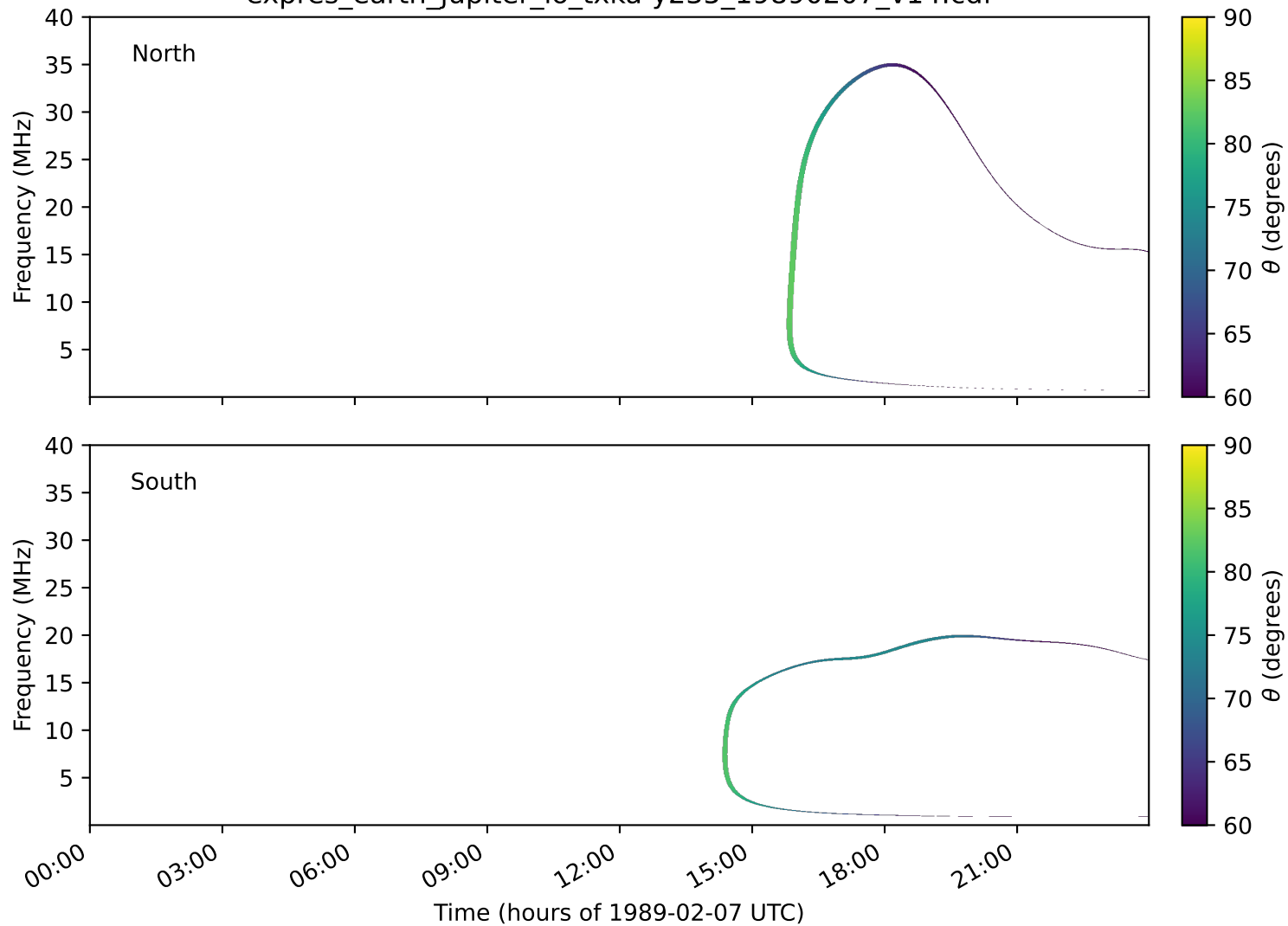
expres_earth_jupiter_io_txka-y235_19890207_v14.cdf
