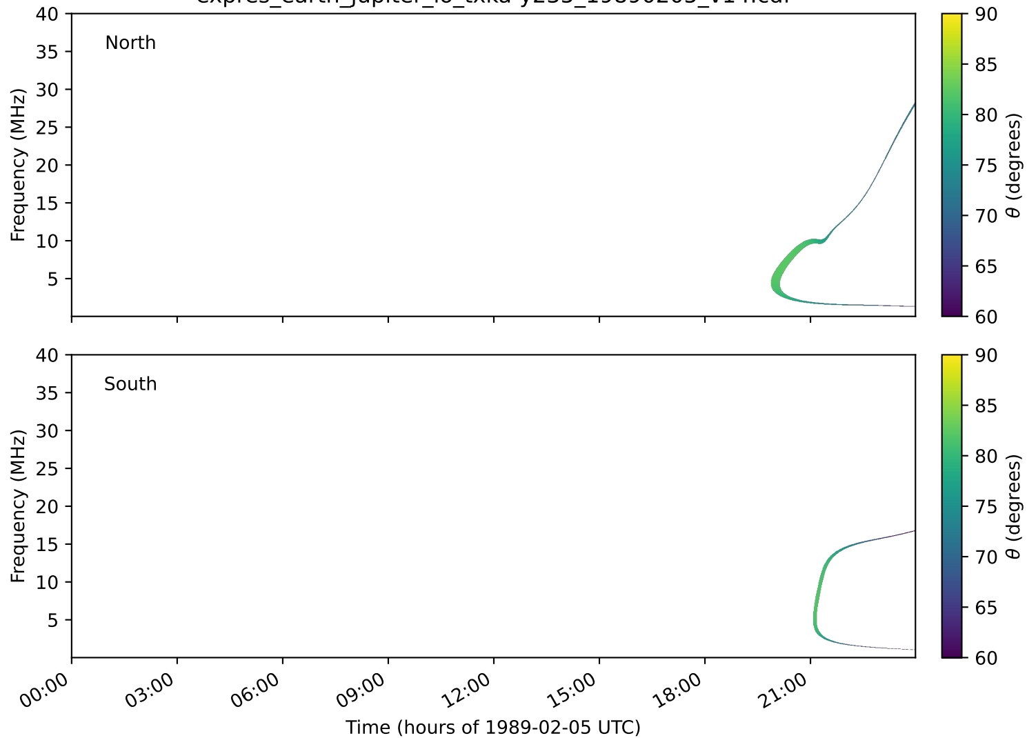
expres_earth_jupiter_io_txka-y235_19890205_v14.cdf
